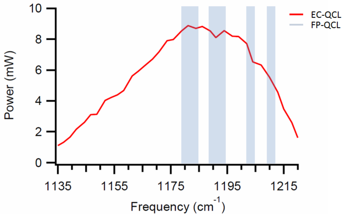
Figure 1.5: Tuning range comparison for Fabry-Pérot and external-cavity quantum cascade lasers. The red trace shows the useful tuning range of the external cavity quantum cascade laser, while the blue bars represent accessible ranges for the Fabry-Pérot laser. Note that while the Fabry-Pérot laser had sizeable coverage gaps, the external-cavity laser had continuous frequency coverage in this region. Figure adapted from Gibson et al. [31].
